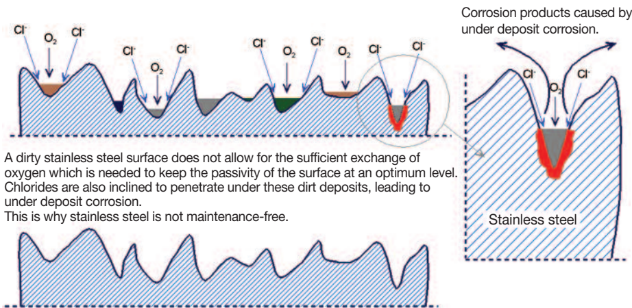
Fig. 7. Diagrammatic representation of dirt in pores and its consequences for a stainless steel surface.
