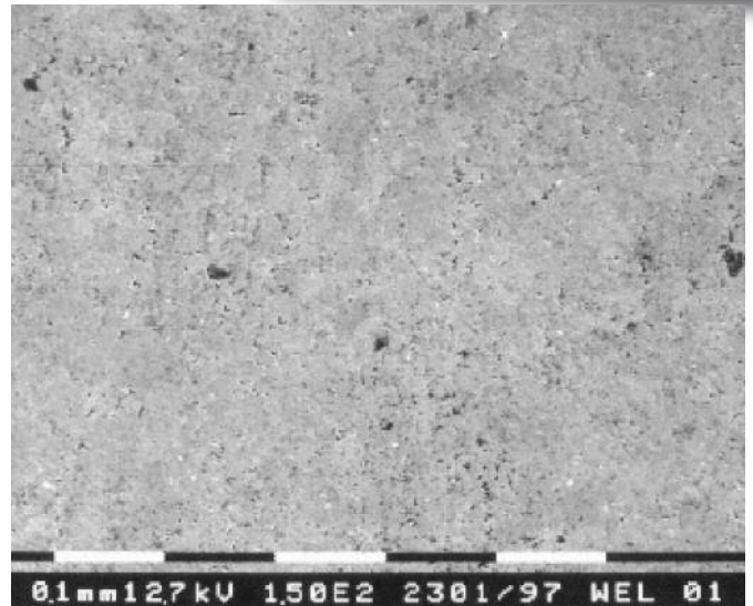
Fig. 6. The same surface as in Fig. 5 after electrolytic polishing (V = 1500x). Photo by Dockweiler Nederland b.v.
