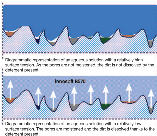
Fig. 9. Diagrammatic representation of effect achieved through a low surface tension
