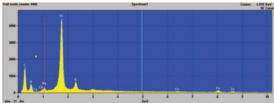
Fig. 2. EDX analysis of dirt in pores of stainless steel.
