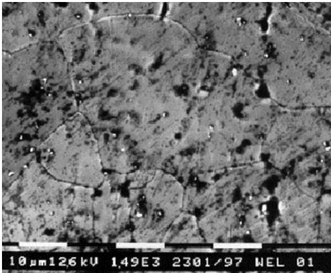
Fig. 5. Dirt pockets are clearly visible on the stainless steel surface (V = 1500x). Photo by Dockweiler Nederland b.v.
